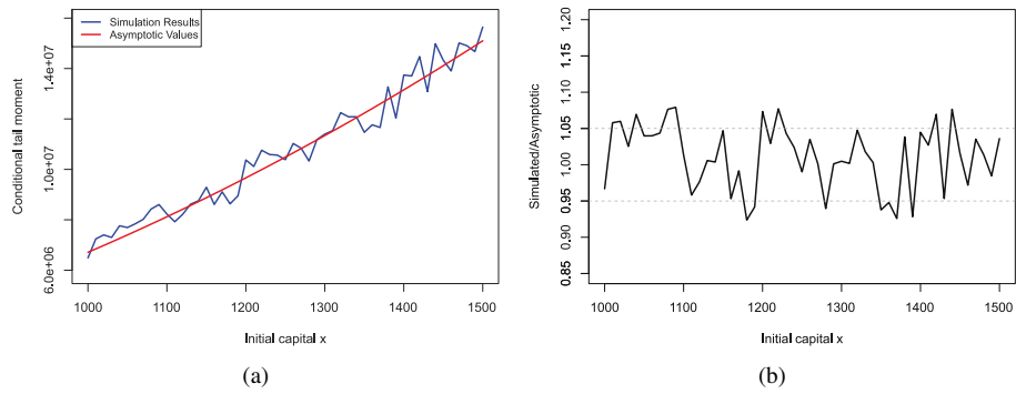
Figure 2. Comparison between the simulated and the asymptotic values of \mathbf{E}[S_n^T | S_n > x] (a) and their ratio (b) via the Gumbel copula.
