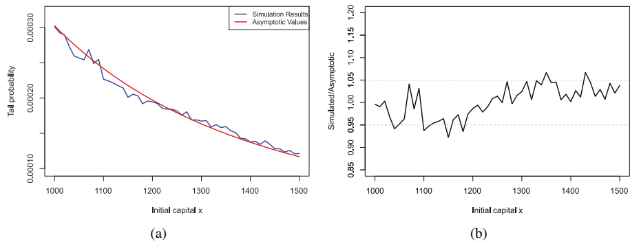
Figure 1. Comparison between the simulated and the asymptotic values of \mathbf{P}(S_n > x) (a) and their ratio (b) via the Gumbel copula.
