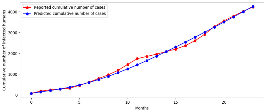
Figure 4. Cumulative number of leptospirosis cases in Kerala from January 2021 to December 2022: predicted vs. actual data.
