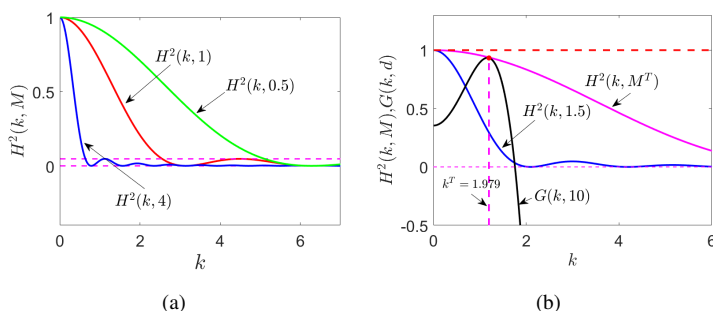
Figure 4. (a) The graphs of the function h = h(kM) for M = 4 , M = 1 , M = 0.5 . (b) For 0 < d < d_c , there exists M^T such that G(k, d) and h(kM^T) are tangent at k = k^T . Here a = 20 , m = 6 , c = 5 , and d = 10 .
