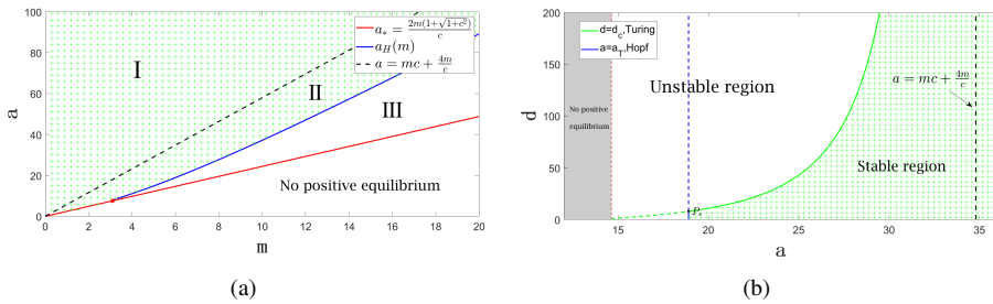
Figure 2. a) The positive equilibrium E_+ of the ODE (5) is asymptotically stable for (m, a) \in I \cup II and unstable for (m, a) \in III ; (b) stable region and bifurcation diagrams in a, d -plane for system (26) with m = 6 , c = 5 . The black dotted line is the vertical asymptotic line of the curve d = d_c .
