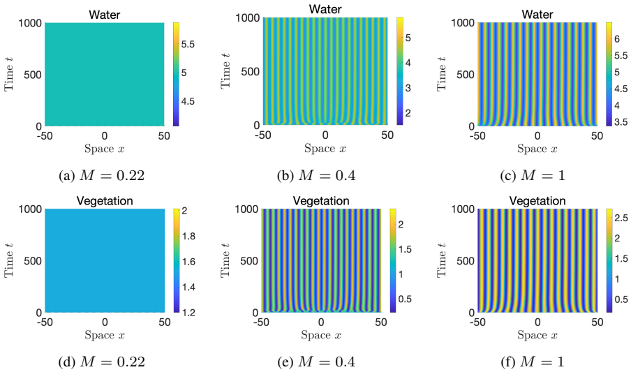
Figure 6. (a) and (d) E_+ is stable for M = 0.22 < M^T ; (b) and (e) E_+ is unstable for M = 0.4 > M^T ; (c) and (f) E_+ is unstable for M = 1 > M^T .
