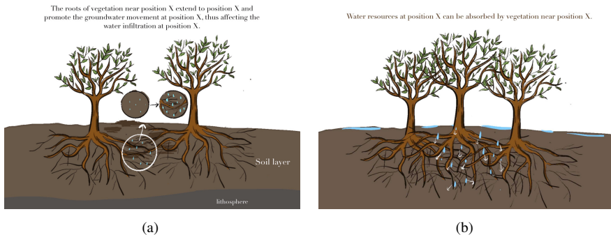
Figure 1. (a) Nonlocal infiltration; (b) nonlocal absorption.
