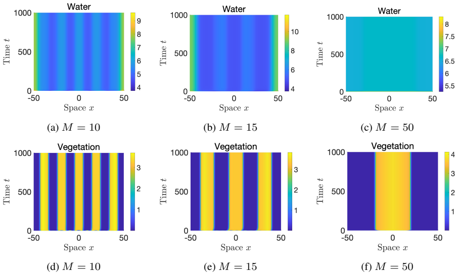
Figure 7. Spatial patterns for system (4) with nonlocal terms (43) for M far from the critical value M^T .
