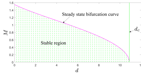
Figure 5. Stability region and bifurcation diagrams in the d, M -plane for system (4) with the nonlocal terms (43) for a = 20 , m = 6 , and c = 5 .
