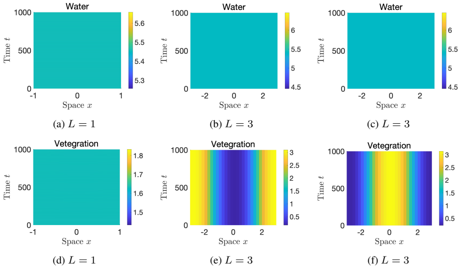
Figure 3. (a) and (d) E_+ is asymptotically stable for L = 1 < L_c ; (b) and (e) for L = 3 > L_c , there exists mode-1 spatially inhomogeneous steady state; (c) and (f) for L = 3 > L_c and the initial functions different from those used in (b) and (e), there exists another mode-1 spatially inhomogeneous steady state.
