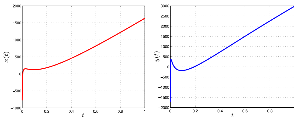
Figure 3. Trajectory of the solution for system (33), (36).
