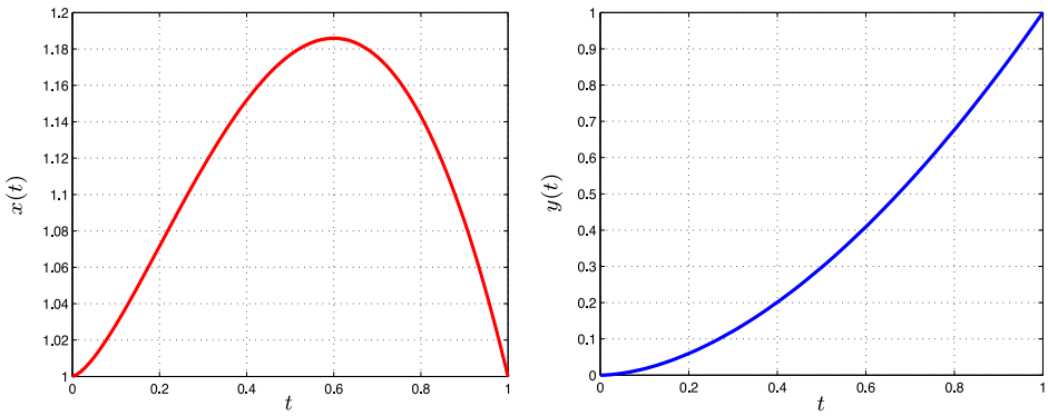
Figure 1. Trajectory of the solution for system (33), (34).
