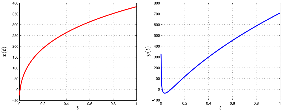
Figure 2. Trajectory of the solution for system (33), (35).
