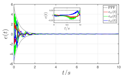
Figure 6. Synchronization errors of systems (23) and (24) without forced impulse.
