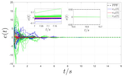
Figure 10. Synchronization errors of systems (25) and (26) without prescribed performance.
