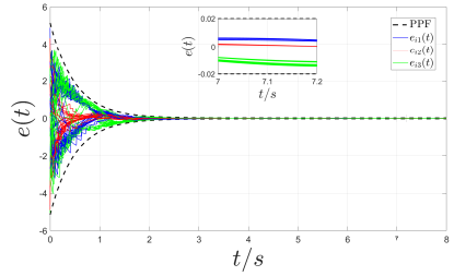
Figure 11. Synchronization errors of systems (25) and (26) without forced impulse.
