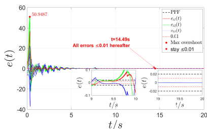
Figure 5. Synchronization errors of systems (23) and (24) without prescribed performance.
