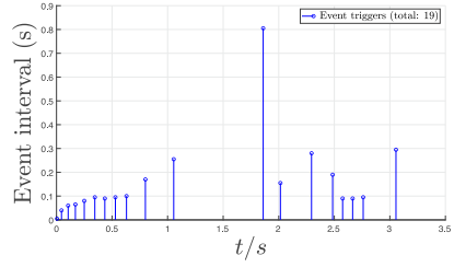
Figure 9. Event-triggering instants and intervals of system (26).
