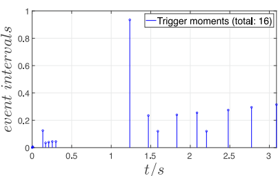
Figure 4. Event-triggering instants and intervals of system (24).
