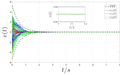
Figure 8. Synchronization errors of systems (25) and (26) with prescribed performance.
