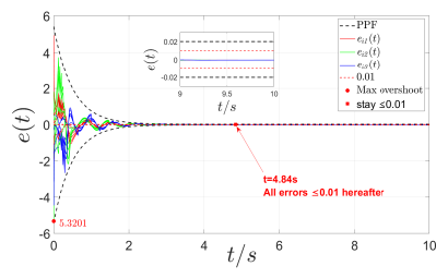
Figure 3. Synchronization errors with prescribed performance.
