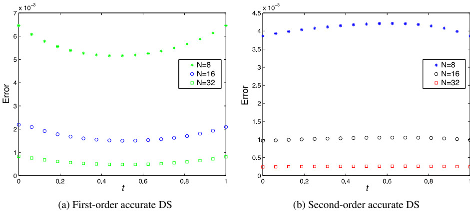
Figure 2. Error in the L_{2h} -norm at the same points with different numbers of discretization N .
