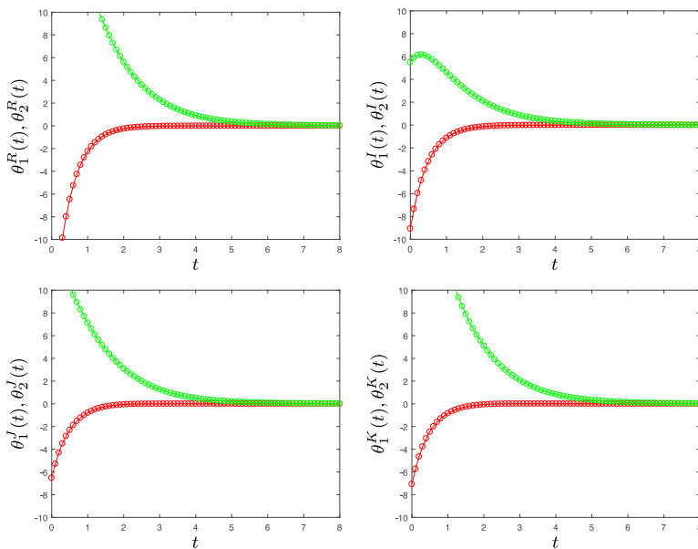
Figure 1. Time evolution of \theta(t) .
